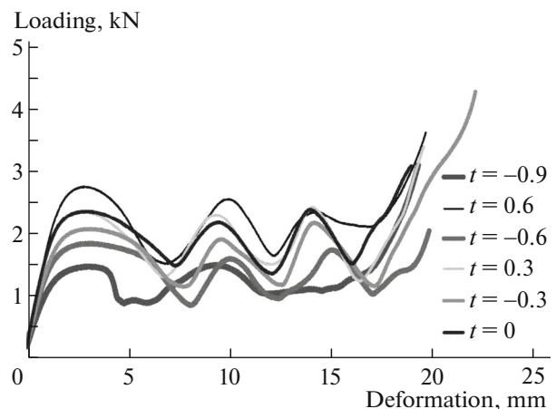
Fig. 2. Stress–strain curves.
