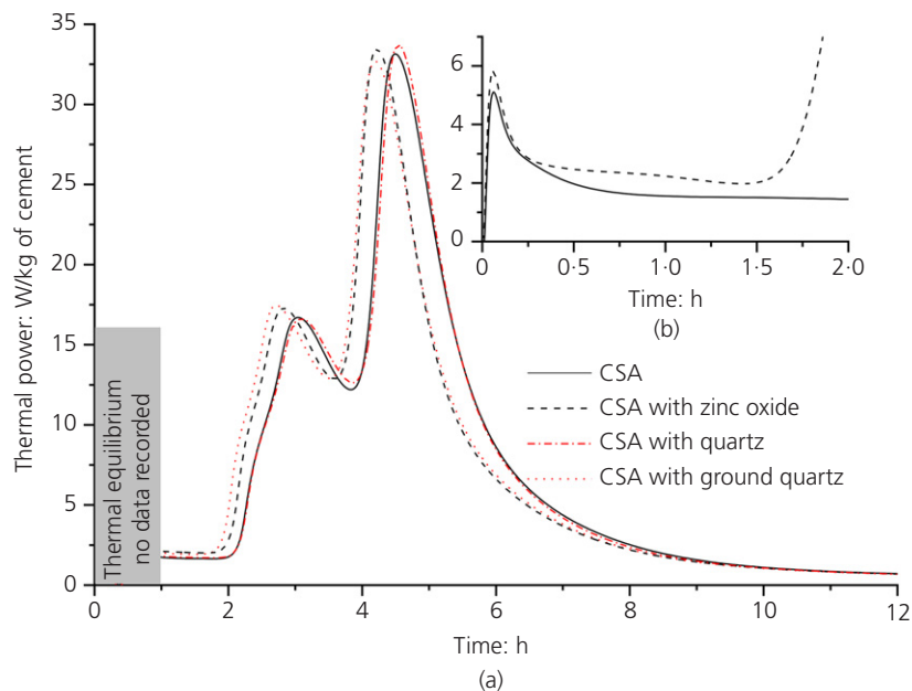
Figure 4. Heat flow development of mixtures with CSA cement and different fillers as a function of time: (a) between 0 and 12 h using external mixing; (b) (inset) between 0 and 2 h using internal mixing
