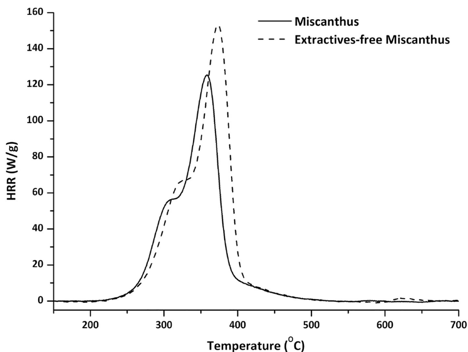
Fig. 5. HRR curves for miscanthus fibers before and after removal of extractives.
