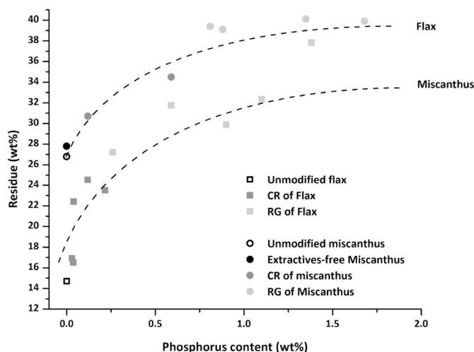
Fig. 17. Variation of residue percentage at 750 °C (anaerobic degradation - TGA) as a function of phosphorus content for miscanthus and flax fibers modified by condensation reaction (CR) and radiation grafting (RG) with VPA.
