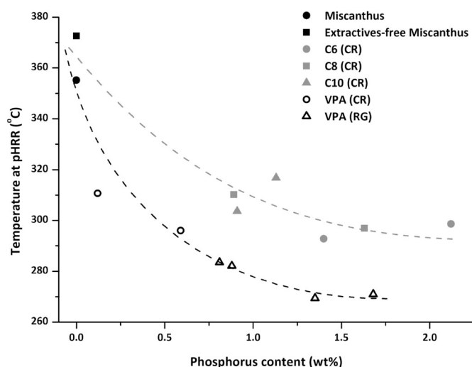
Fig. 13. Variation in pHRR temperature as a function of phosphorus content for miscanthus fibers and those modified by condensation reaction (CR) and radiation grafting (RG) with C6, C8 and C10 bisphosphonic acids and VPA.
