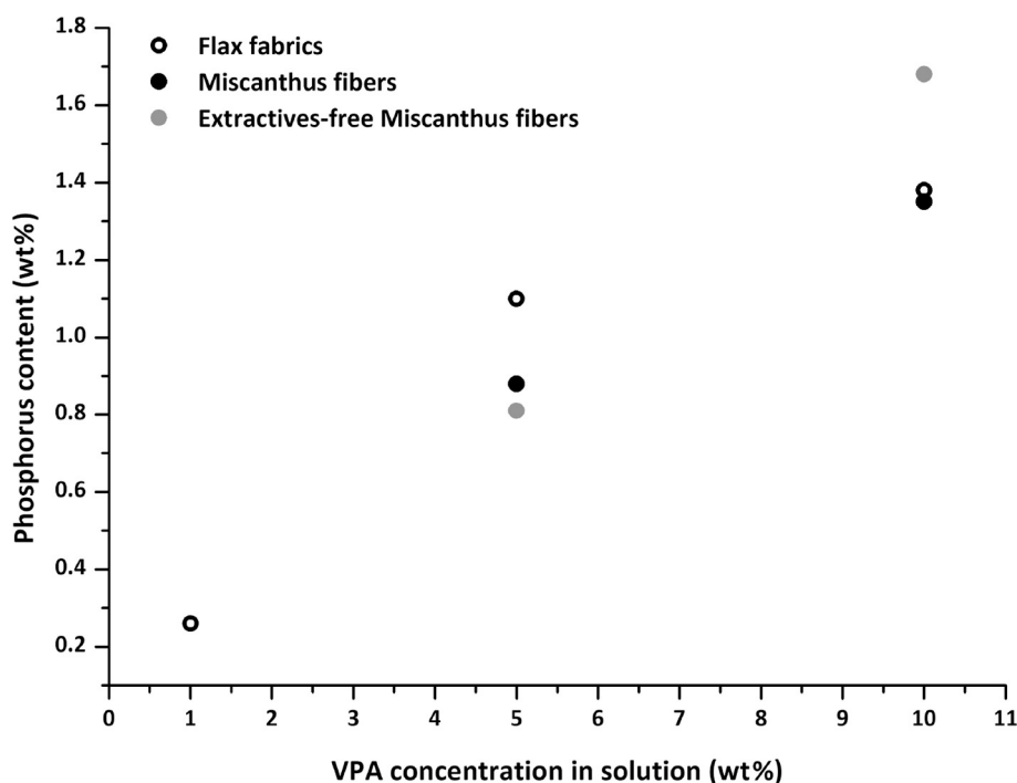
Fig. 2. Phosphorus content of flax fabrics and miscanthus fibers modified by radiation grafting (phosphorus contents for flax fabrics are extracted from previous studies [20,21])
