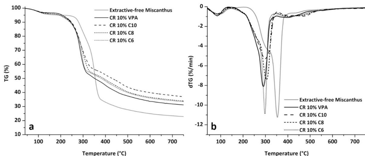
Fig. 9. TGA (a) and dTG (b) curves for miscanthus fibers and for miscanthus fibers modified by condensation reaction (CR) under mild conditions with a 10 wt% solution of VPA, C10, C8 or C6.
