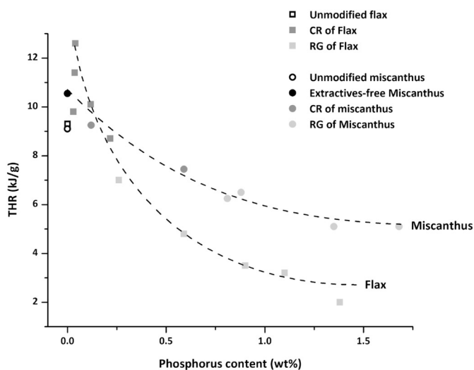
Fig. 16. Variation of total heat release (THR) as a function of phosphorus content for miscanthus and flax fibers modified by condensation reaction (CR) and radiation grafting (RG) with VPA.
