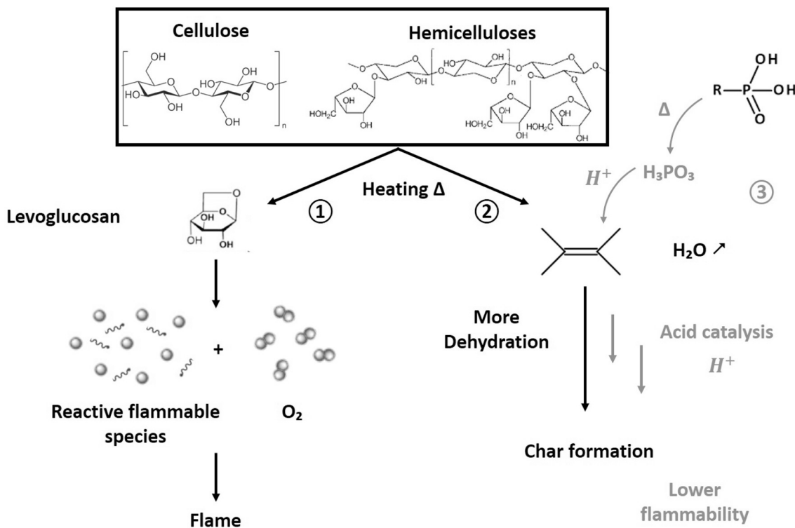
Scheme 1. Mechanism of degradation of cellulosic material by 1) depolymerization, 2) dehydration and 3) promotion of mechanism 2 in presence of phosphonic flame retardant.
