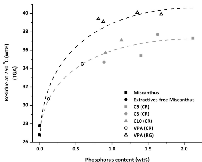
Fig. 15. Variation of the residue percentage at 750 °C compared to the dry mass of the fibers (anaerobic degradation - TGA) as a function of the phosphorus content for miscanthus fibers and those modified by condensation reaction (CR) and radiation grafting (RG) with C6, C8 and C10 bisphosphonic acids and VPA.
