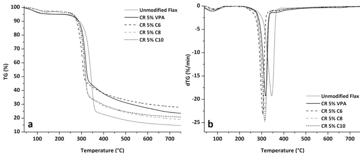
Fig. 11. TGA (a) and dTG (b) curves for unmodified flax fibers and for flax fibers modified by condensation reaction (CR) under mild conditions with a 5 wt% solution of VPA, C6, C8 or C10.
