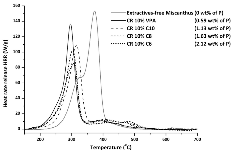
Fig. 8. HRR curves for miscanthus fibers and for miscanthus fibers modified by condensation reaction (CR) under mild conditions with a 10 wt% solution of VPA, C10, C8 or C6.
