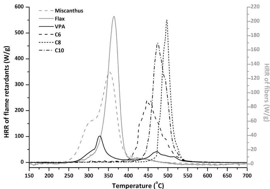
Fig. 12. HRR curves for miscanthus and flax fibers and molecules used for modification.
