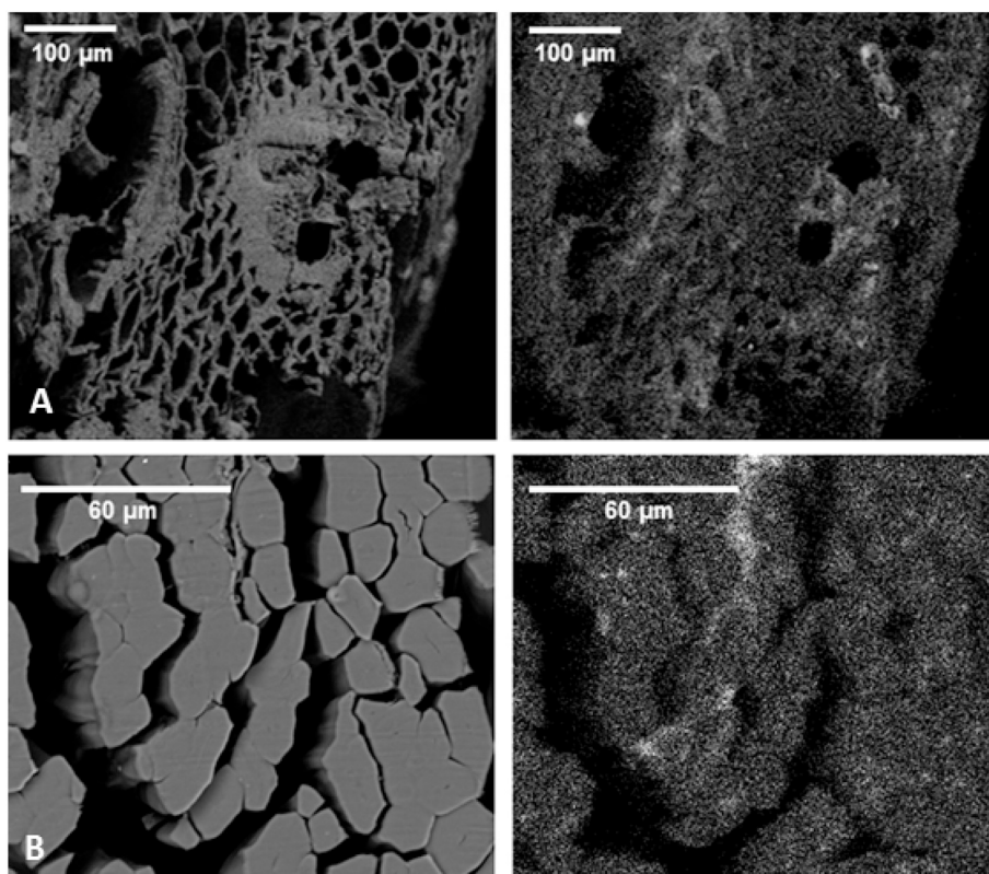
Fig. 4. SEM images (left) and EDX phosphorus mapping (right) of miscanthus fibers (A) and flax fibers (B) treated with solutions of 5 wt% C6 bisphosphonic acid aqueous solutions by chemical modification under mild conditions
