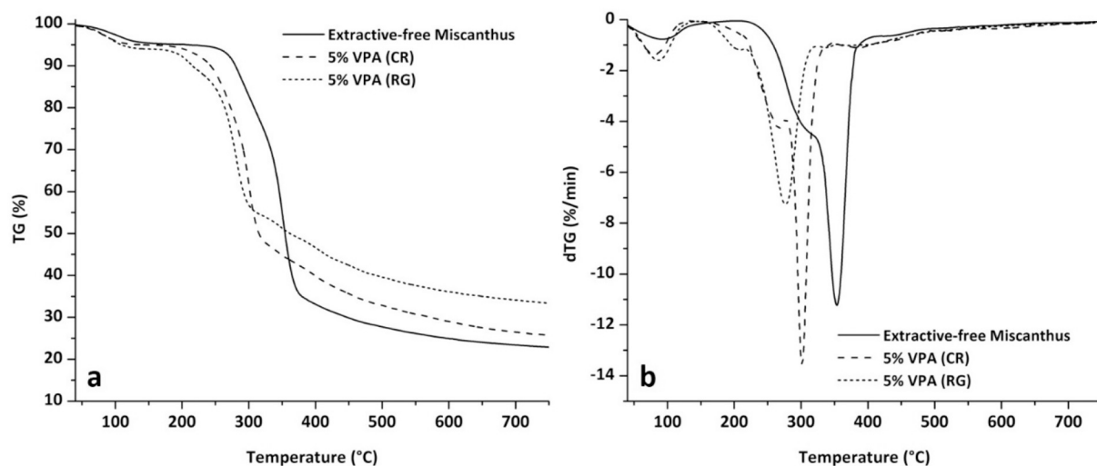
Fig. 6. TGA (a) and dTG (b) curves for miscanthus fibers, miscanthus fibers modified by condensation reaction (CR) under mild conditions and by radiografting (RG) at 50 kGy with a 5 wt% VPA solution.
