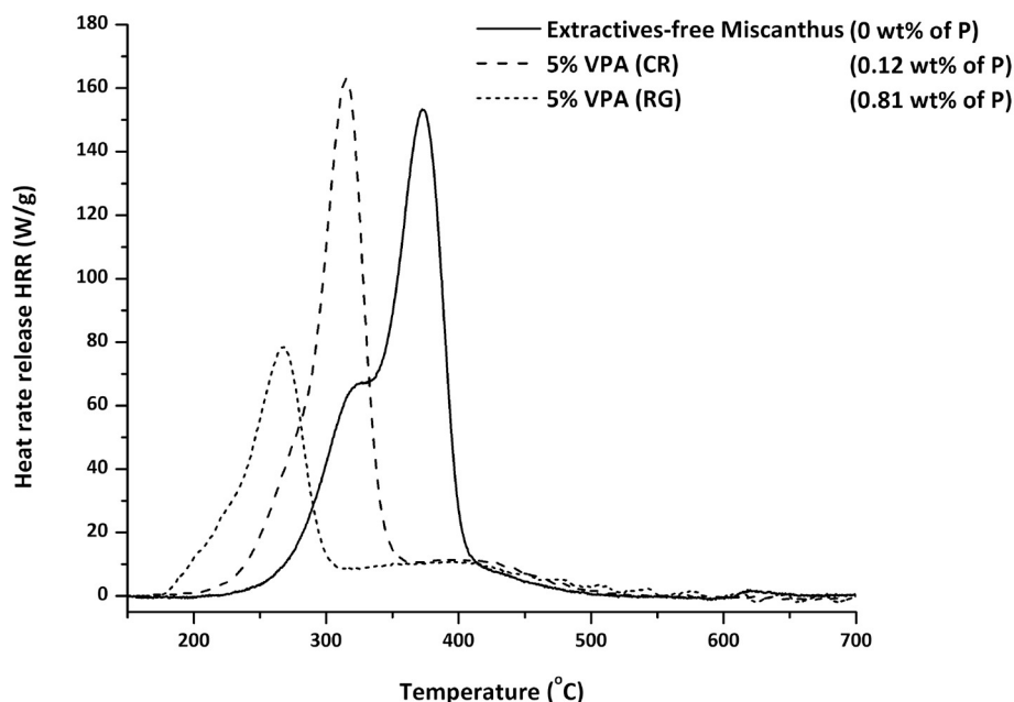
Fig. 7. HRR curves for miscanthus fibers, miscanthus fibers modified by condensation reaction (CR) under mild conditions and by radiografting (RG) at 50 kGy with a 5 wt% VPA solution.
