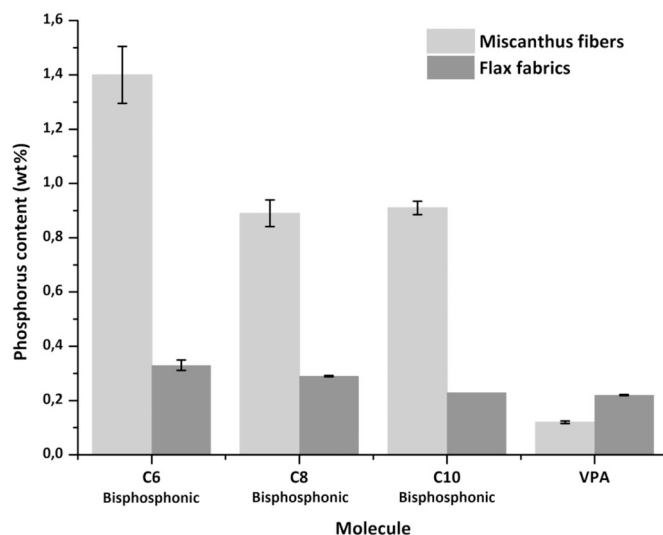
Fig. 3. Variation in the phosphorus content grafted on miscanthus fibers and flax fabrics by condensation reaction under mild conditions with 5 wt% of the bisphosphonic molecules in the reaction solution.
