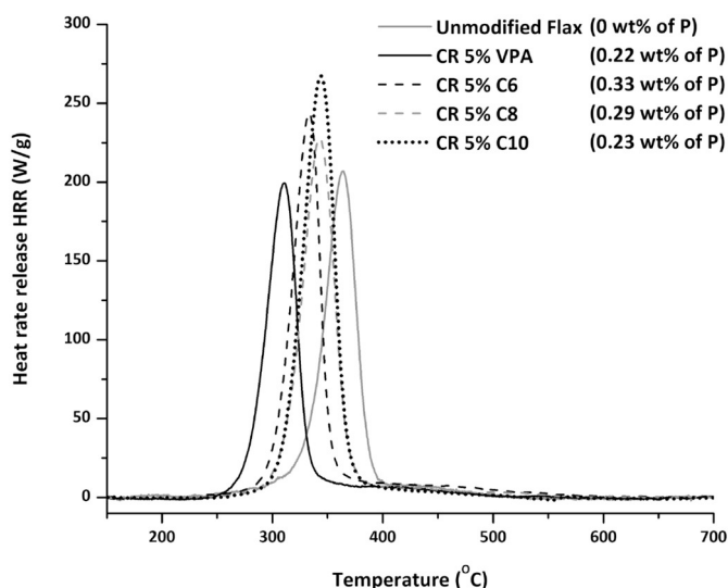
Fig. 10. HRR curves for unmodified flax fibers and for flax fibers modified by condensation reaction (CR) under mild conditions with a 5 wt% solution of VPA, C6, C8 or C10.
