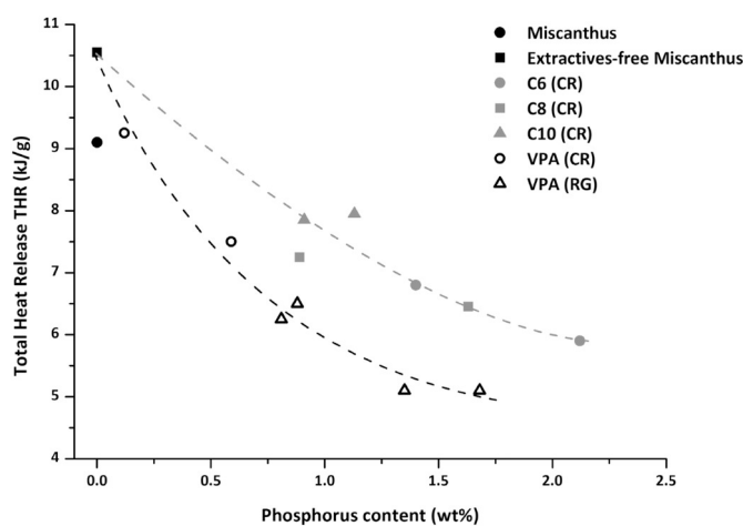
Fig. 14. Variation of total heat release (THR) as a function of phosphorus content for miscanthus fibers and those modified by condensation reaction (CR) and radiation grafting (RG) with C6, C8 and C10 bisphosphonic acids and VPA.
