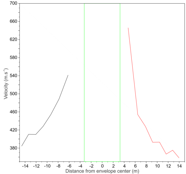
Figure 11: Blast waves velocity outside the envelope. Colors refer to corresponding rectangle in figure 10. In order to smooth uncertainties on blast wave position at each time step, velocity is computed between 30 images. Green lines illustrate geometrical the limits of the initial envelope.
