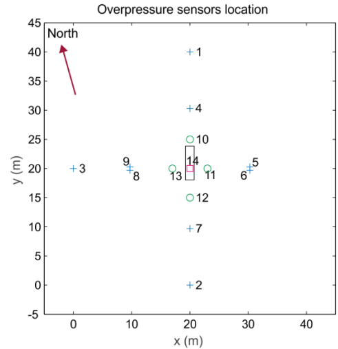
Figure 2 : Location of overpressure sensors Altitude of the sensors is respectively 0.88 m, 1.80 m, and 1.95 m for o, + and □.
