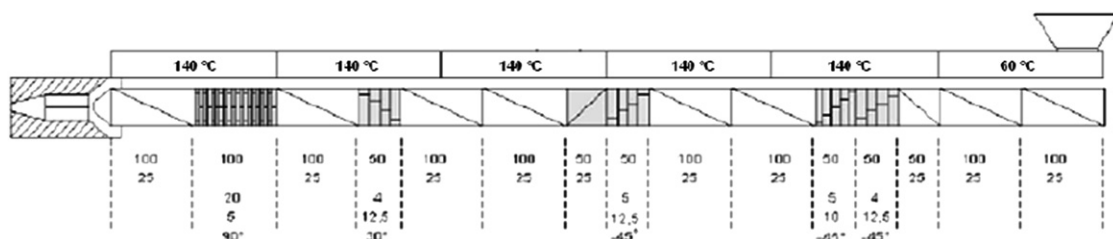
Fig. 1. Screw Configuration.
