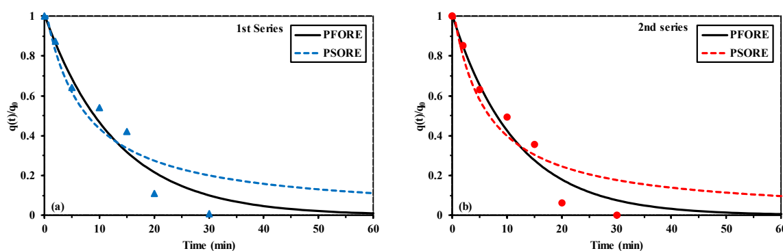
Figure 6. Desorption kinetics for U(VI) loaded on Q-APEI—Modeling with the PFORE and the PSORE for the 1st series (a) and the 2nd Series (b) (samples collected from uptake kinetics; eluent: 0.5 M NaCl/0.5 M HCl; SD: 0.85 g L -1 ; agitation speed: 170 rpm; T: 22 ± 2 °C).
