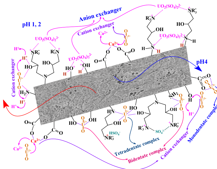
Scheme 1. Tentative mechanism for U(VI) sorption on Q-APEI.
