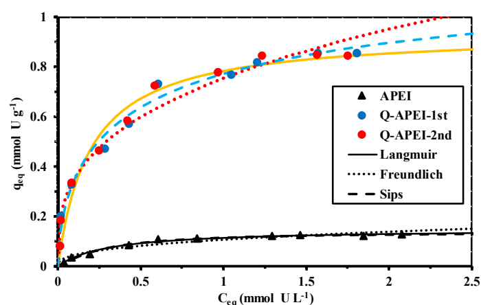
Figure 5. U(VI) sorption isotherms at pH 4 using APEI and Q-APEI—Modeling with the equations of Langmuir, Freundlich, and Sips (SD: 0.375 \text{ g L}^{-1} ; \text{pH}_0 : 4; \text{pH}_{\text{eq}} : 3.87–3.69 for Q-APEI and 4.19–3.97 for APEI; C_0 : 0.04\text{--}2.13 \text{ mmol U L}^{-1} ; agitation speed: 170 rpm; contact time: 48 h; T : 22 \pm 2 \text{ }^\circ\text{C} ).
