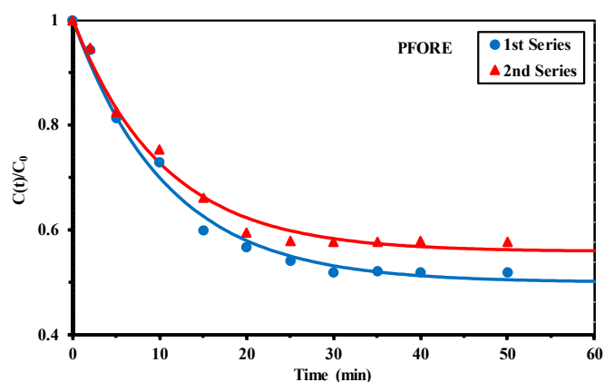
Figure 4. U(VI) uptake kinetics using Q-APEI sorbent—Modeling with the pseudo-first order rate equation (PFORE) (SD: 0.3\text{ g L}^{-1} ; \text{pH}_0 : 4; \text{pH}_{\text{eq}} : 3.79–3.71; C_0 : 0.214\text{ mmol U L}^{-1} and 0.249\text{ mmol U L}^{-1} for the 1st and 2nd series, respectively; agitation speed: 170 rpm; T: 22 \pm 2\text{ }^\circ\text{C} ).
