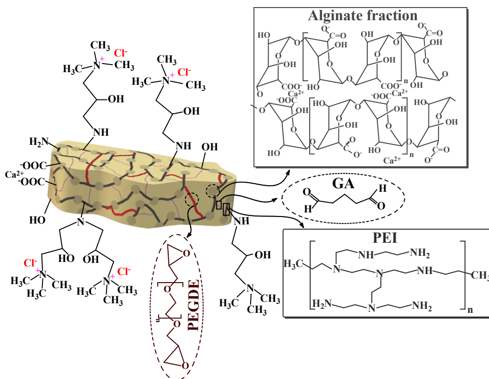
Scheme 2. Structure of the sorbent.
