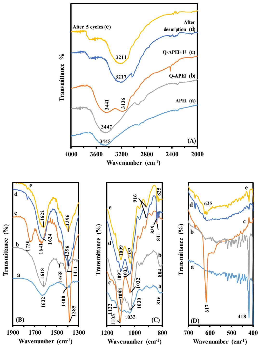
Figure 1. FTIR spectra (selected wavenumber ranges).
