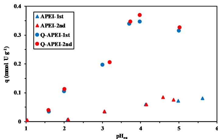
Figure 3. Effect of pH on U(VI) sorption using APEI and Q-APEI sorbents (Sorbent dosage (SD): 0.333 \text{ g L}^{-1} ; contact time: 48 h; agitation speed: 170 rpm; T: 22 \pm 2 \text{ }^\circ\text{C} ).
