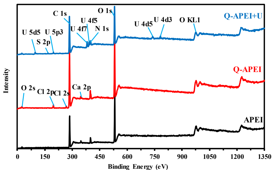
Figure 2. XPS survey of raw material (APEI), after modification (Q-APEI), and after uranium sorption (Q-APEI-U).
