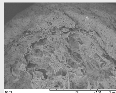
Figure 2. SEM of (PLA + Arbocel) foam cross section exhibiting outer skin and layered structure.
