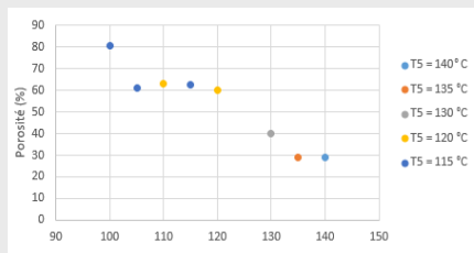
Figure 1. Porosity as a function of die temperature T 6 for different pre-expansion temperature T s for PLA mixture extrusion-foaming
