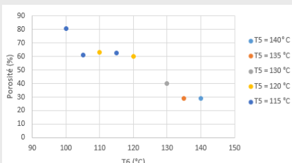
Figure 1. Porosity as a function of die temperature T 6 for different pre-expansion temperature T s for PLA mixture extrusion-foaming
