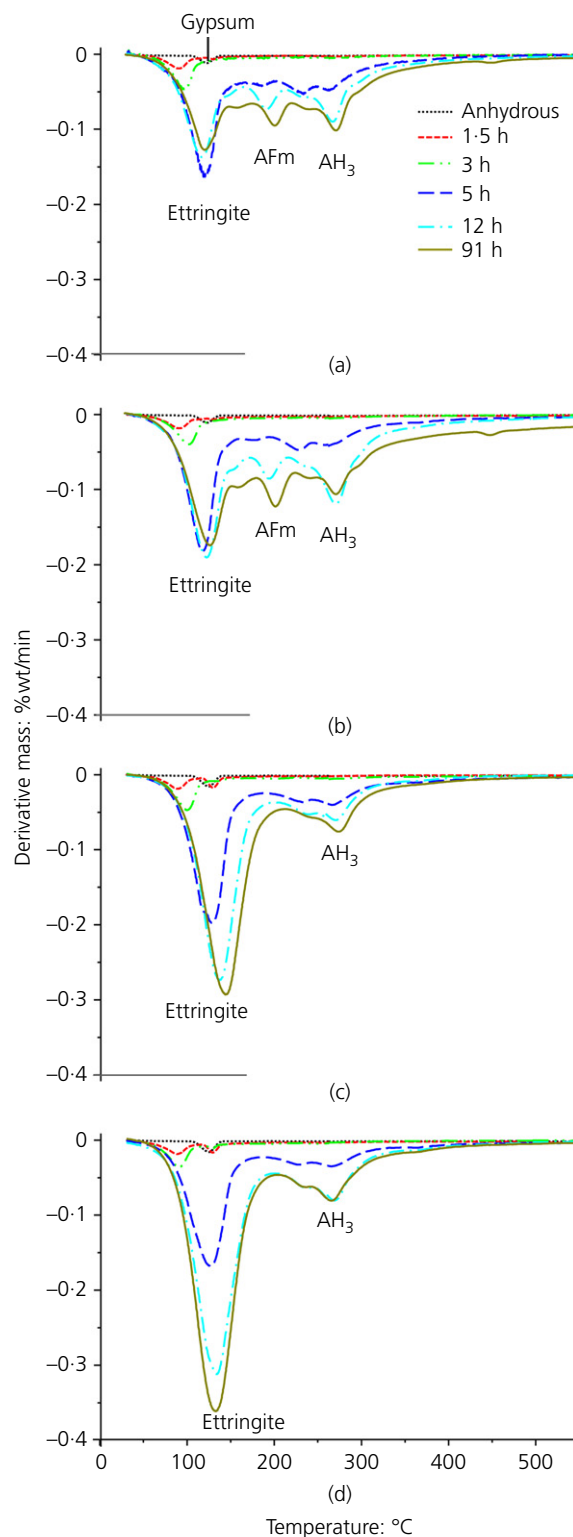
Figure 5. Differential TGA data for (a) T3W4, (b) T3W7, (c) T5W4 and (d) T5W7 pastes
