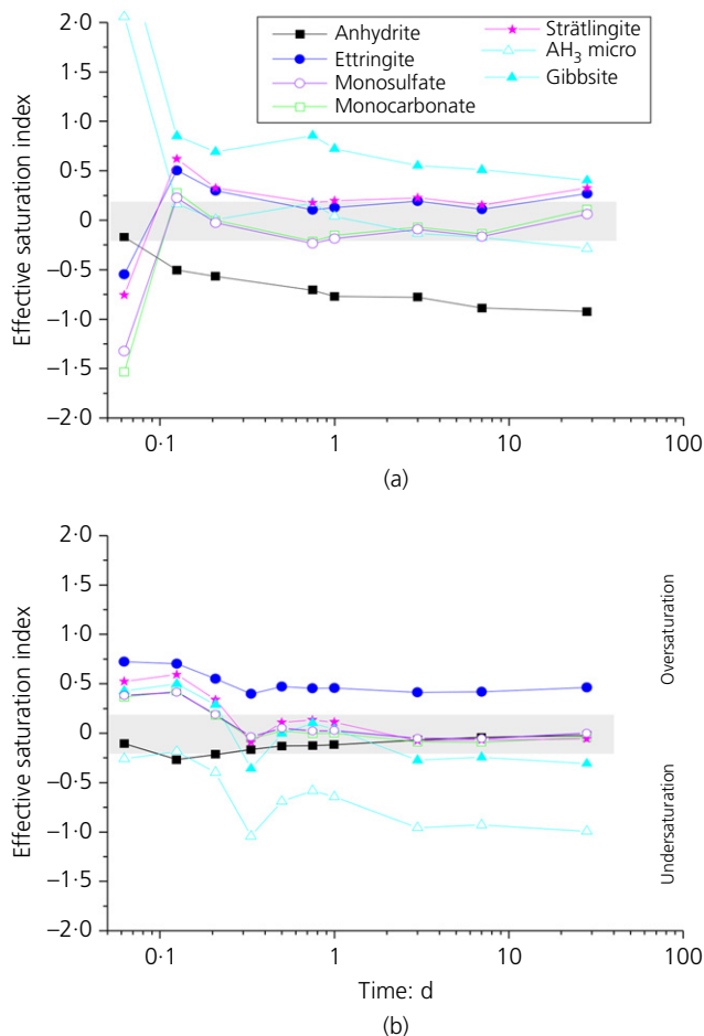
Figure 8. Effective saturation indices of anhydrite, ettringite, AFm phases (monosulfate, monocarbonate), strätlingite and AH 3 micro of hydrated pastes (a) T3W7 and (b) T5W7 as a function of time. The shadowed area indicates saturation
