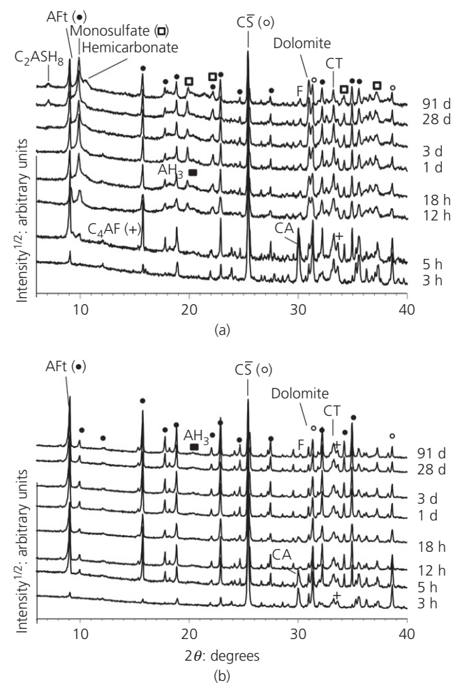
Figure 4. Diffraction patterns of (a) T3W7 and (b) T5W7 between 6 and 40°, CuK\alpha
