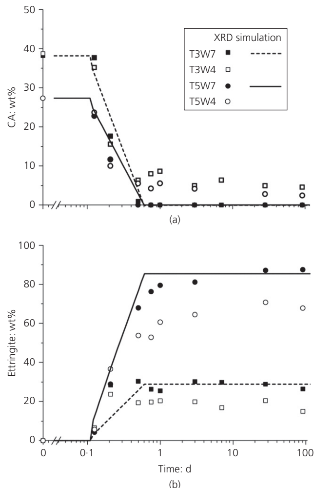
Figure 9. Amount of CA used as input in the thermodynamic model (a) and ettringite (b) deduced by XRD/Rietveld analysis as a function of hydration time. Lines refer to the results of thermodynamic modelling
