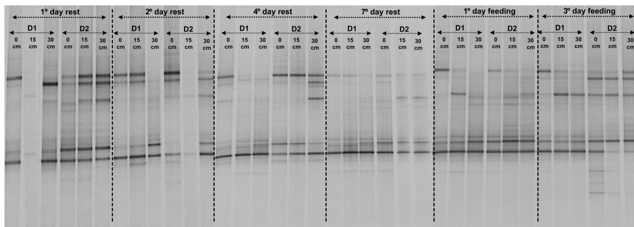
Figure 3. Temporal and spatial DGGE profiles of a nitrifying (AOB) bacterial community in S3. d1 = 1 m from the feeding point; d2 = 2 m from the feeding point; 0, 15 and 30 cm depth.
