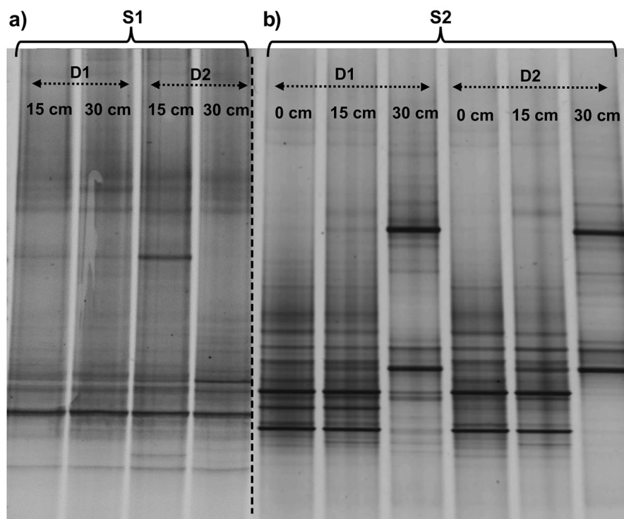
Figure 2. DGGE gel banding temporal and spatial profiles of nitrifying (AOB) bacterial communities in systems (a) S1 and (b) S2. d_1 = 1 m from the feeding point; d_2 = 2 m from the feeding point; 0, 15 and 30 cm depth. Each black line represents a band that corresponds to a group of AOB.
