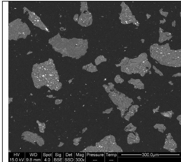
Figure 8 : ESEM observation of polished cross section of 20% PMC(<400μm) filled PP (x300)
