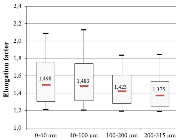
Fig. 17 Elongation factor of different PMC size fractions measured by image analysis (central line: median value, upper/lower corner of the box : d_{75}/d_{25} , upper/lower bounds : d_{90}/d_{10} )
