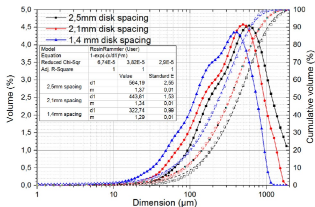
Fig. 13 Laser PSD of micronized PMC (disk mill) for different disk spacing. Hollow dots represent measured cumulative PSD, dashed lines correspond to RR fit
