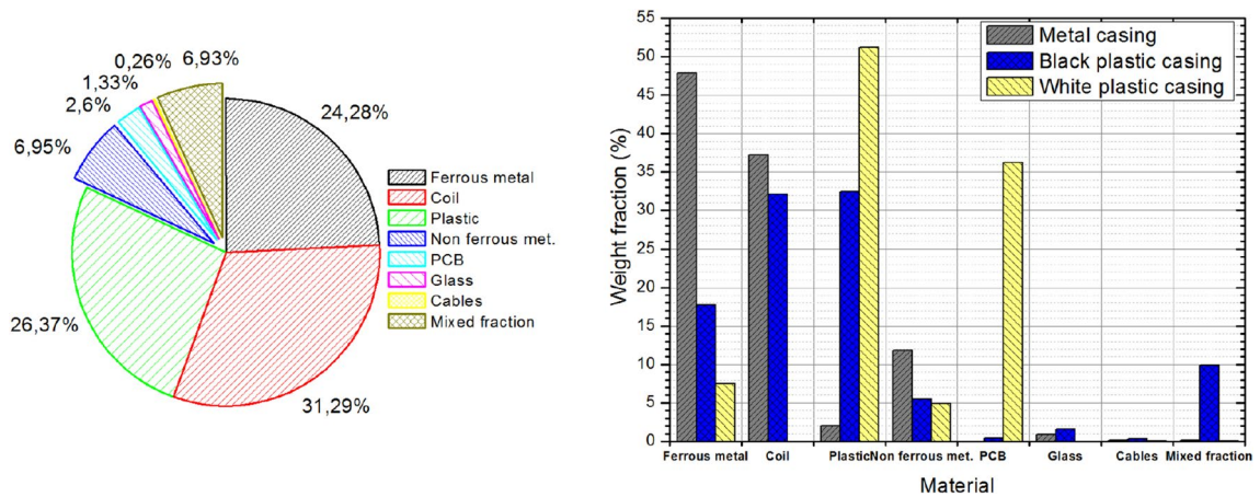
Fig. 5 Mass repartition of materials in the whole sample (left) and per EM type (right)
