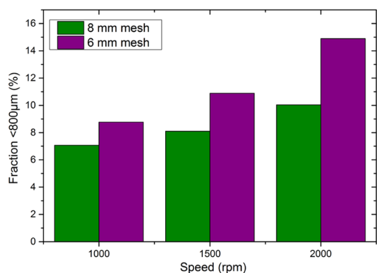
Fig. 12 Fine fraction (<800 µm) production in a knife mill as a function of knife speed and grid size
