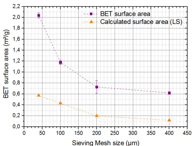
Fig. 15 BET surface area of sieved powder as a function of sieving mesh size (Square: measured; Triangle: equivalent spherical surface calculated from laser scattering PSD)
