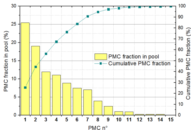
Fig. 7 Mass fraction of each PMC part in the overall PMC pool
