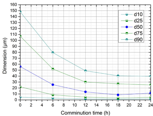
Fig. 19 Particle size distribution measured by laser diffraction of PMC comminuted in a ball mill during different times (second ball set milling time)
