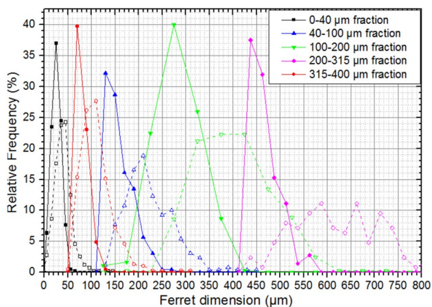
Fig. 16 Minimum (solid line, full dots) and maximum (dashed line, hollow dots) ferret diameter of five fraction of particles measured by image analysis
