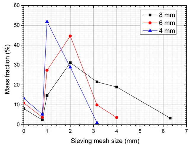
Fig. 11 Mass PSD of PMC crushed with a knife mill with 3 sizes of grid, measured by sieving (1500 rpm)
