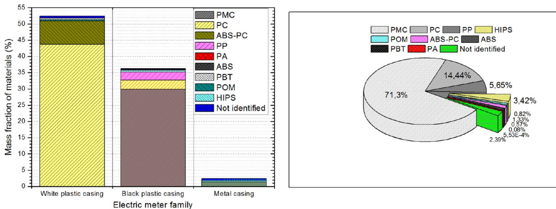
Fig. 6 Mass fraction of plastics in the different type of electrical meter (left) and composition of plastics in the overall sample (right)
