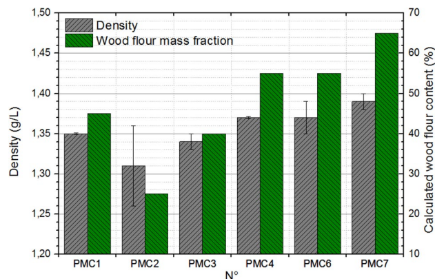
Fig. 9 Measured densities of PMC and calculated wood flour content
