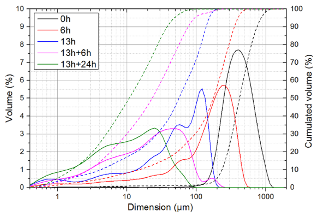
Fig. 18 Particle size distribution measured by laser diffraction of PMC comminuted in a ball mill during different times (First ball set milling time + second ball set milling time)
