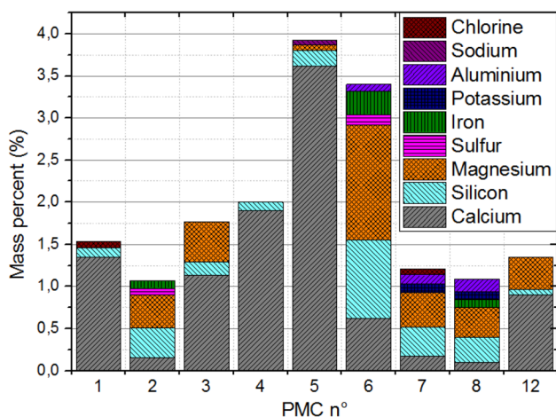
Fig. 8 Elemental analysis of the PMC formulation by EDX
