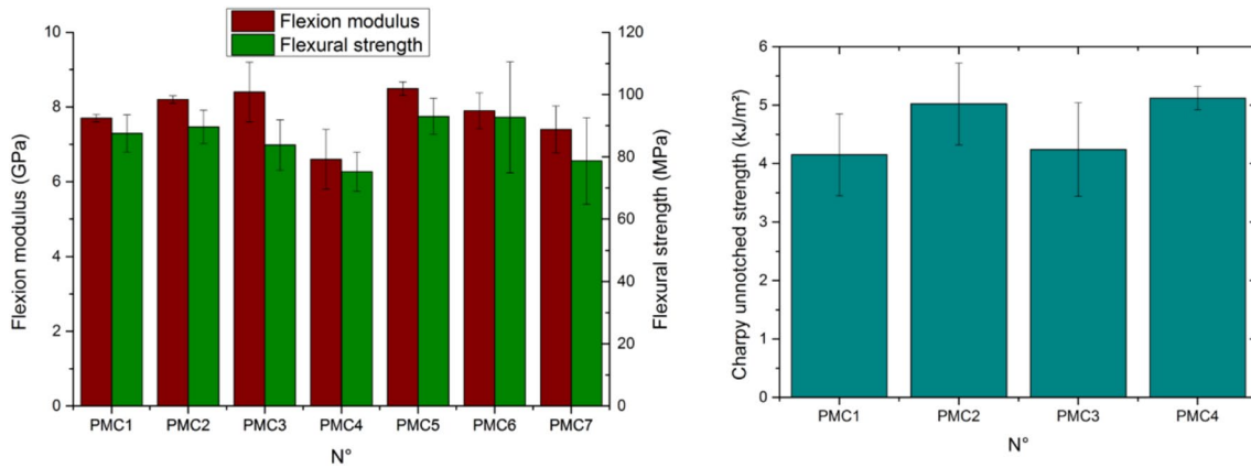
Fig. 10 Flexural modulus and strength (left) and Charpy impact strength (right) of PMC
