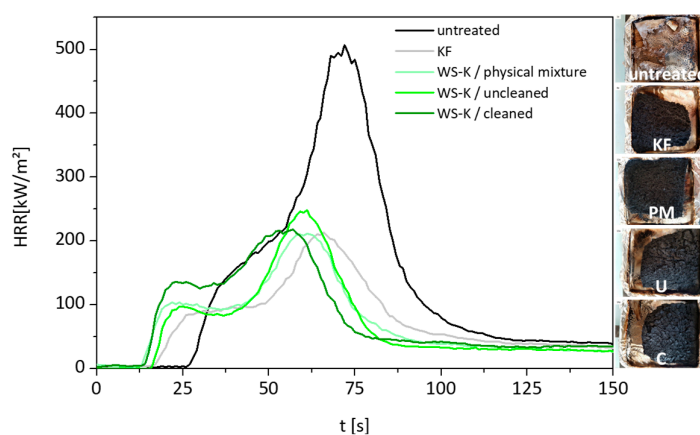
Figure 7. Left, heat release rate curves from CC measurement of untreated wood fibers without additive (reference), with commercial flame retardant KF and starch-based WS-K in form of physical mixture (PM), uncleaned (U) and cleaned synthesis product (C); right, photos of the residues from the cone calorimeter tests.
