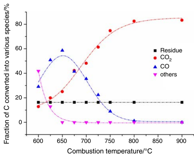
Fig. 11 Fraction of carbon converted into different species versus the combustion temperature for sheath from cable C
