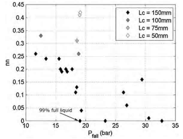
Fig. 24. Exponent nn vs burst pressure for 2017 results.
