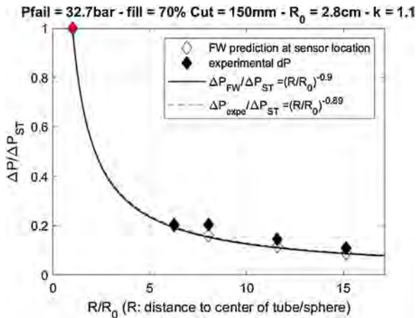
Fig. 13. ΔP s /ΔP st vs R/R 0c for Test 23.
