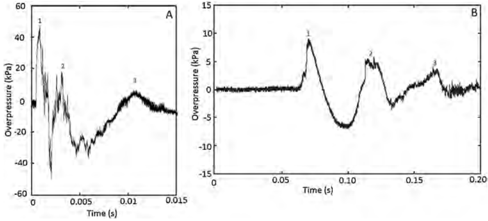
Fig. 6. Typical examples of BLEVE blast waves from propane BLEVEs. On the left is a sample from an aluminum 0.6 L tube BLEVE R = 25.4 mm with L = 300 mm ( P_{fail} = 28 bar, fill_{liq} = 63\% , measured 29 cm above the vessel). On the right is a BLEVE of a 2000 l propane tank ( P_{fail} = 18 bar, fill_{liq} = 49\% , measured at 20 m on the side of the vessel) (Birk et al., 2007) 1) lead shock, 2) second overpressure from vapour space release, 3) overpressure (not shock) from liquid flashing.
