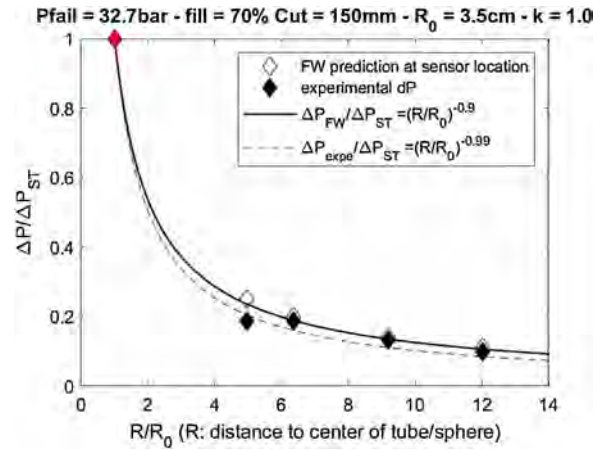
Fig. 16. adjusted result for Test 23, k = 1, R_0 = 0.0354 m from full tube length L = 300 mm.
