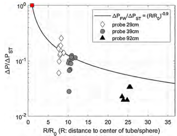
Fig. 19. May 2015 results with R_0 based on sphere.
