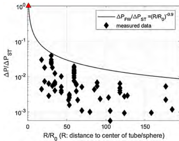
Fig. 28. Peak blast overpressure, British Gas BLEVE tests (Johnson and Pritchard, 1991), various failure pressures and fill levels, 5.7 and 10.8 m³, Butane and Propane, failure on top by shaped charge.
