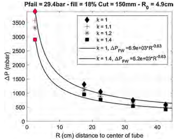
Fig. 15. Variation in Result with k for Propane (test 25).
