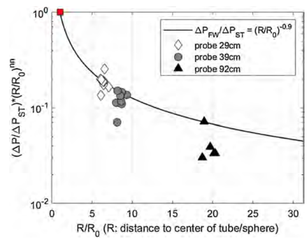
Fig. 25. 2015 Results adjusted with nn for each test to fit the decay curve.
