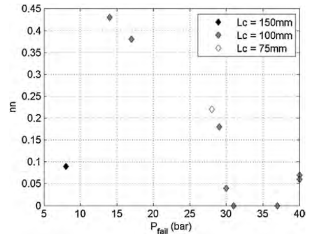
Fig. 26. 2015 Results, exponent nn vs P_f .
