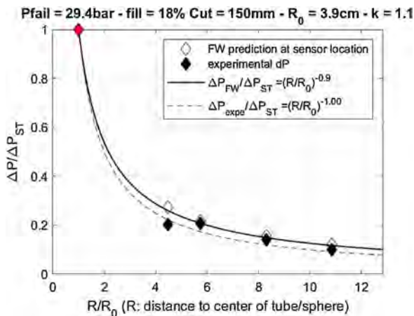
Fig. 14. ΔP s /ΔP st vs R/R 0c for Test 25.
