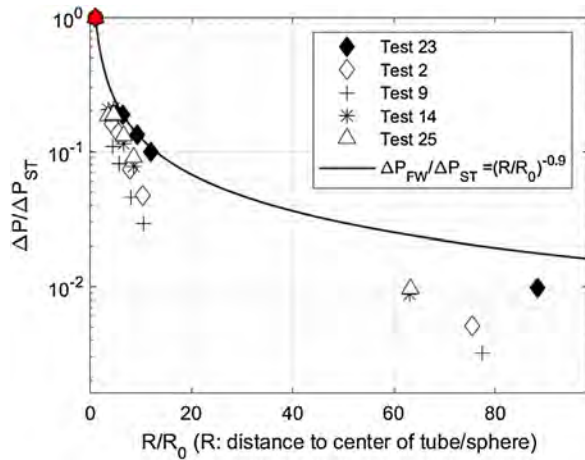
Fig. 18. Peak Overpressure on top from 0.6 L aluminum tube, near and far field, Solid line from FW Theory. All tests with semi-log plot.
