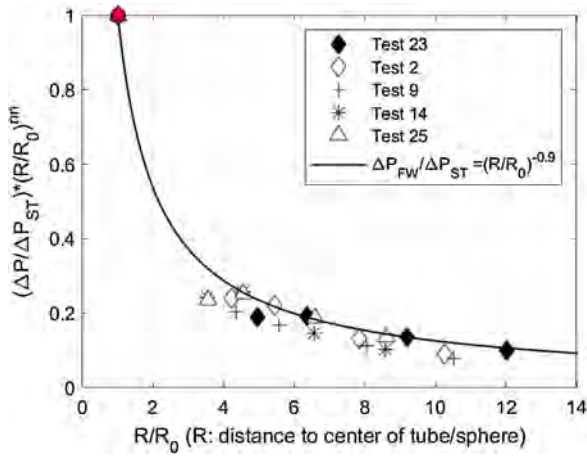
Fig. 22. 2017 results, overpressure data adjusted to fit curve for each test – near field.
