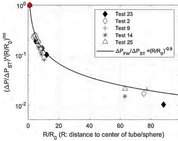
Fig. 23. 2017 results, overpressure data adjusted to fit curve for each test – near and far field.
