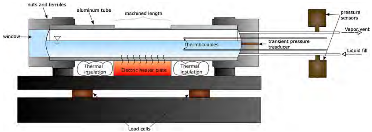
Fig. 5. Schematic diagram of tube apparatus (tube D =50 mm).
