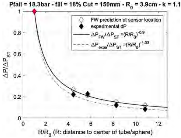
Fig. 12. ΔP s /ΔP st vs R/R 0c for Test 14.
