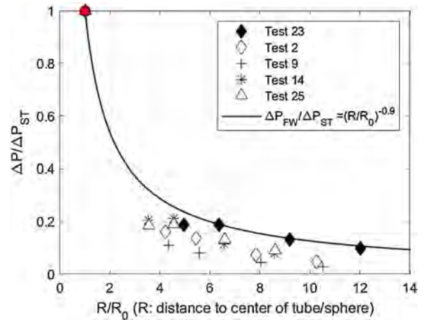
Fig. 17. Peak Overpressure on top from 0.6 L aluminum tube, near and far field, Solid line from FW Theory. All tests.
