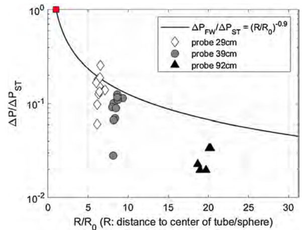
Fig. 20. May 2015 results with R_{oh} based on hemisphere.
