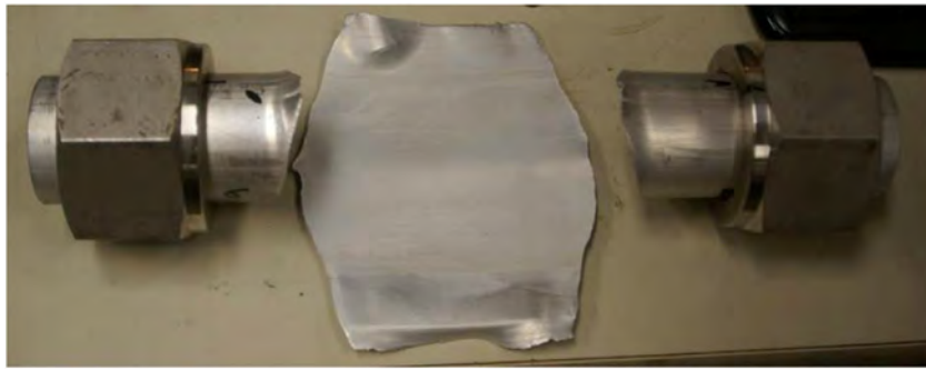
Fig. 2. image of failed tube with separated part of wall flattened on blast plate. Weakened length is the upper and lower free edges of the flattened part.
