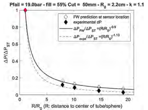
Fig. 11. \Delta P_s/\Delta P_{st} vs R/R_0 for Test 9 (partial opening).
