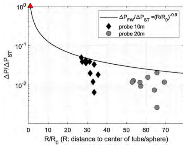
Fig. 27. peak blast overpressure data from (Birk et al., 2007) for 0.4 m³ tank, propane, various failure pressures and fill levels, failure on top by fire exposure.
