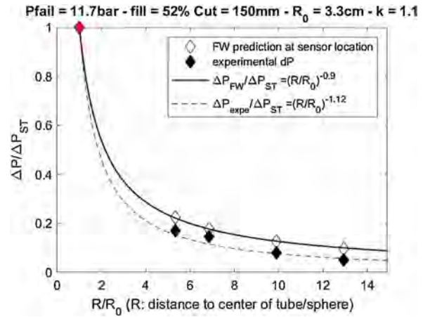
Fig. 10. \Delta P_s/\Delta P_{st} vs R/R_0 for Test 2.
