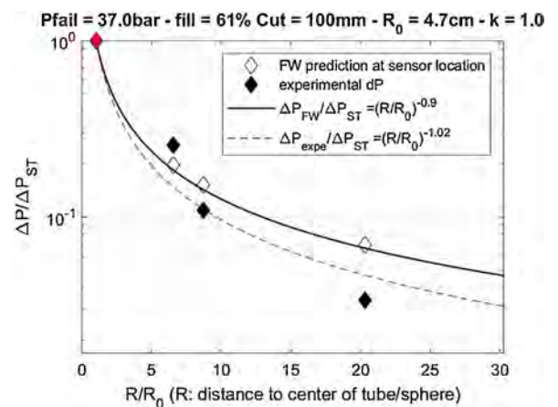
Fig. 21. May 2015, test 12 with R_{oh} based on hemisphere.
