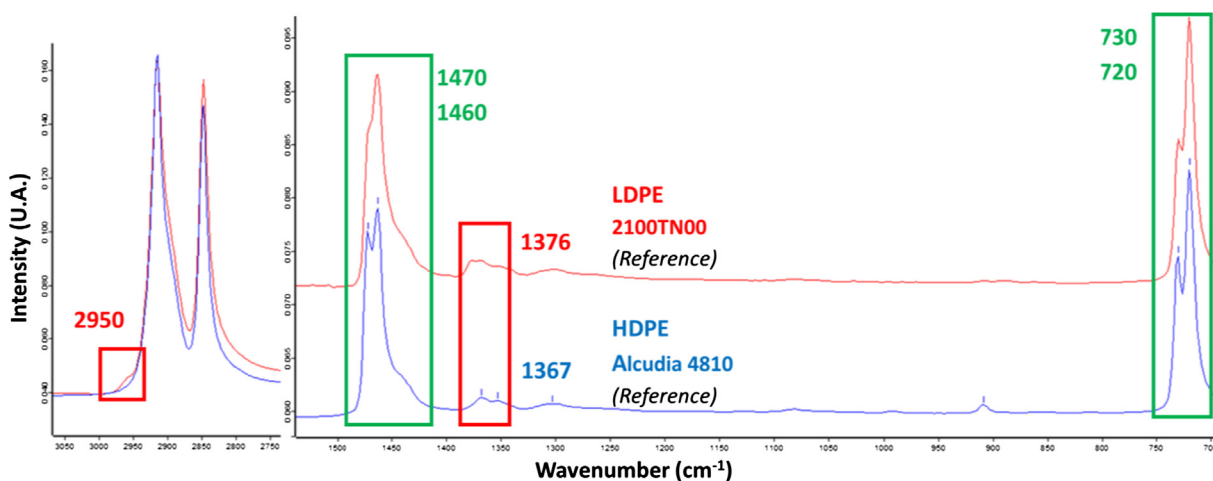
Fig. 2. LDPE and HDPE reference samples in MIR – red frames for CH 3 peaks & green frames for crystallinity markers. (For interpretation of the references to color in this figure legend, the reader is referred to the web version of this article.)
