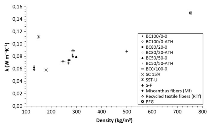
Figure 11. Figure 11 Evolution of thermal conductivity ( \lambda ) of the BCs as a function of density in comparison with the literature (SC15%: sunflower/chitosan-based panels 20 ; SST-U: sunflower stem/stalk fibers/textile waste-urea formaldehyde-based panels 16 ; S-F: sunflower-free binder panels 48 ; PFG: palm fiber gypsum-based panels 49 ).
